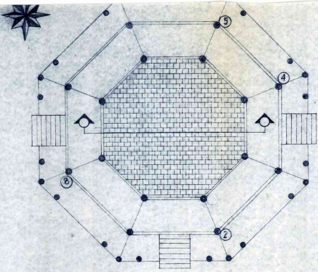
㉔ KEY PLAN S:1/100
